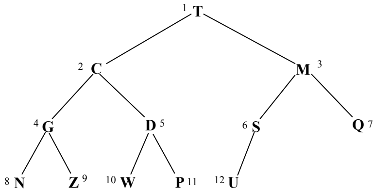
Fig. 54-8 The T leaf has been cut off and placed in the root.
