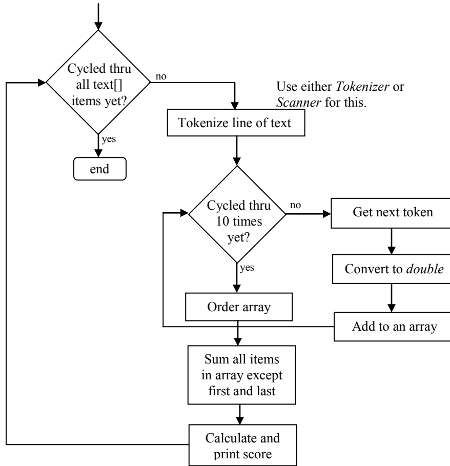
Fig. 26-1 Flow chart for gymnastics project. This assumes the lines of text from the input file have already been stored in the text[ ] array.
